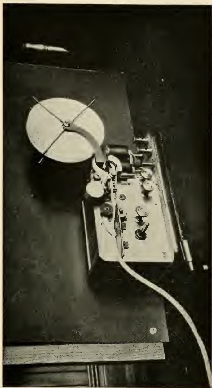
Fig. 16.—The Self-Recording Telegraph Instrument. ( I'ide , p. 228.) (Size .25 diameters.)
